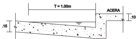
CUNETA TRIANGULAR
