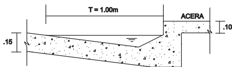
CUNETA TRIANGULAR
