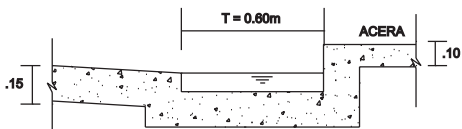
CUNETA RECTANGULAR
